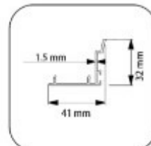
7 - Frame Locking Profile
