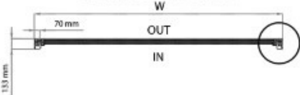
2 PANELS SINGLE GLAZING
