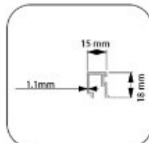
6b - Frame - Glass Fixing Profile (Single Glass)
