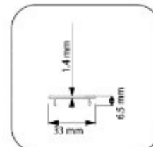
8 - Frame Cap Profile
